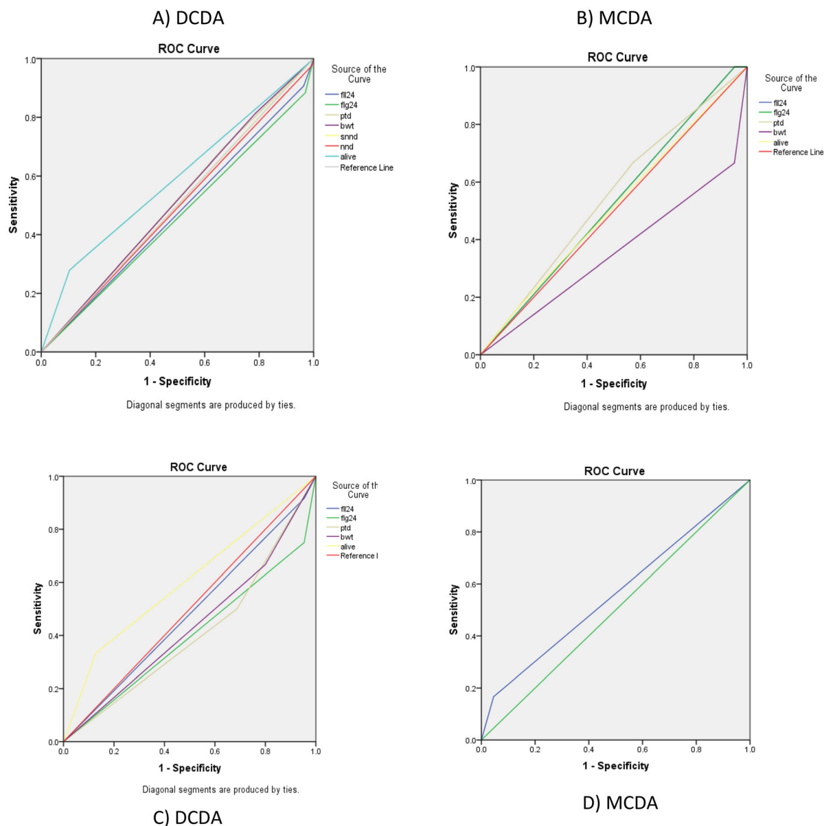
Fig. 1 A, B - ROC curves of DC and MC twins for CRL discordancy \geq 10\% as a predictor of fetal loss < 24 weeks, preterm delivery, birthweight discordance, babies alive after 28 days. C - ROC curves of DC twins for CRL discordancy \geq 16\% as a predictor of fetal loss
